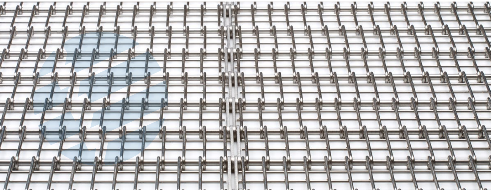
Eye-Flex® with underwelded wire spacing
